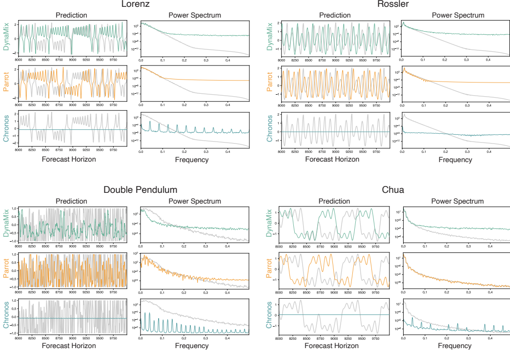
Figure 3: Context parroting best reconstructs the power spectra of chaotic systems despite its predictions being periodic. Predictions of four distinct chaotic systems using the two best-performing models DynaMix and Chronos, relative to Parroting. We set the context length to L = 2000 . Forecasts are generated for 10,000 points past the end of the context, and the last 2000 timepoints are shown. The power spectrum is estimated using Welch’s method on the last 5000 timepoints.
