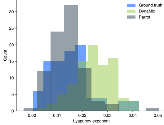
Figure 11: Histograms of Lyapunov Exponents. We estimate the Lyapunov exponents from the ground-truth time series, as well as from long rollouts from parroting and DynaMix, the current-generation foundation model with the best ability to preserve long-term properties. These rollouts are generated with a context length of 2000 and a prediction horizon of 10000, and correspond to estimates from all distinct chaotic systems in dysts .
