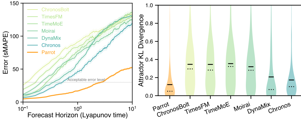
Figure 2: Context parrot outperforms foundation models in zero-shot forecasting for both short-term point-wise accuracy and long-term attractor reconstruction. Left: Forecast error of each model as a function of the forecast horizon. The context length is set to 512 for all models. Right: KL Divergence between the predicted attractors and the true attractors (smaller is better). Solid lines represent mean and dotted lines represent median. All results are obtained from 135 chaotic systems in the dysts database, with 20 trajectories from random initial conditions for each system.
