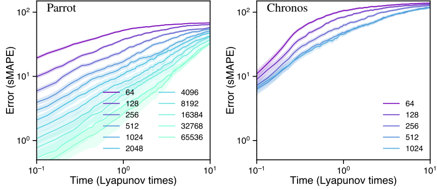
Figure 4: Parroting can better utilize longer context data while Chronos does better for shorter contexts. Each line represents the forecast error for a different context length. The performance of Chronos saturates once the context length exceeds its designed upper limit of 512 data points, whereas the accuracy of context parroting keeps improving for longer context windows. Here we set the embedding dimension D = 5 for the parroting algorithm.
