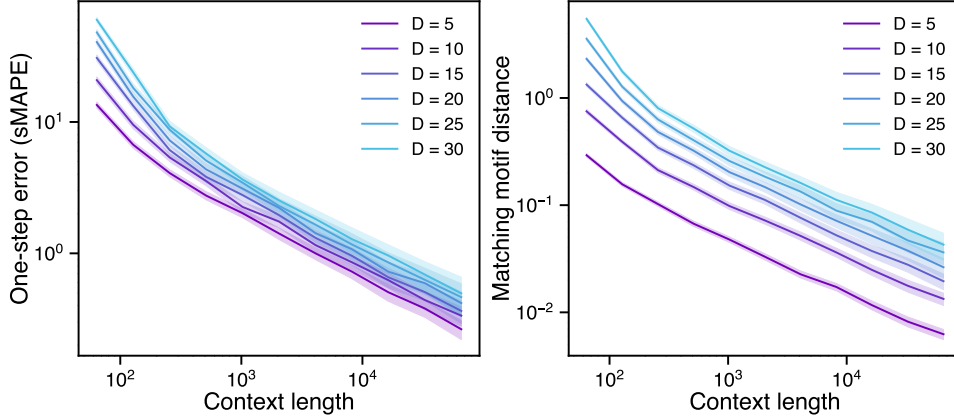
Figure 10: Scaling laws with context length. Left: One-step forecast error versus context length. The scaling follows a power law for all embedding dimensions D considered. Smaller D is more accurate here because of the one-step forecast error. Larger D can be more accurate for longer forecasting horizons. Right: Euclidean distance between the last context motif x_{L-D+1:L} and its closest match, as a function of context length. Again, the scaling follows a power law for all D .
