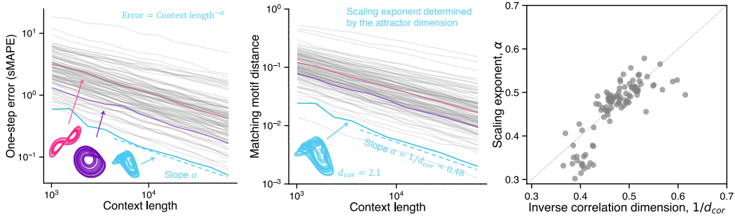
Figure 5: Context parroting explains in-context neural scaling laws and links scaling exponents to attractor dimensions. Left: One-step forecast error versus context length. Each line represents a distinct chaotic system and the scaling follows a power law. In principle, infinite context length should give parroting infinite accuracy for any deterministic system with a well-defined attractor. Middle: Euclidean distance between the last context point and its nearest neighbor in the delay-embedding space, as a function of context length. Again, the scaling follows a power law with the same scaling exponent \alpha . The scaling exponent can be different for each system and is linked to the correlation dimension d_{\text{cor}} of the chaotic attractor through the relation \alpha = 1/d_{\text{cor}} . Right: Estimated scaling exponent \alpha versus the inverse correlation dimension 1/d_{\text{cor}} , where each dot represents a chaotic system. For all panels we set the embedding dimension D = 10 for the parroting algorithm.
